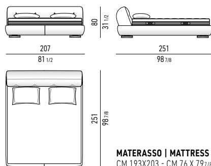
LETTO KING SIZE CM 207X251 BED KING SIZE CM 207X251
